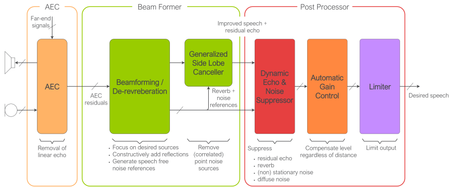
Fig. 4: Voice processing pipeline
