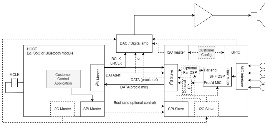
Fig. 2: Functional block diagram of XVF3800 in INT-Device configuration
