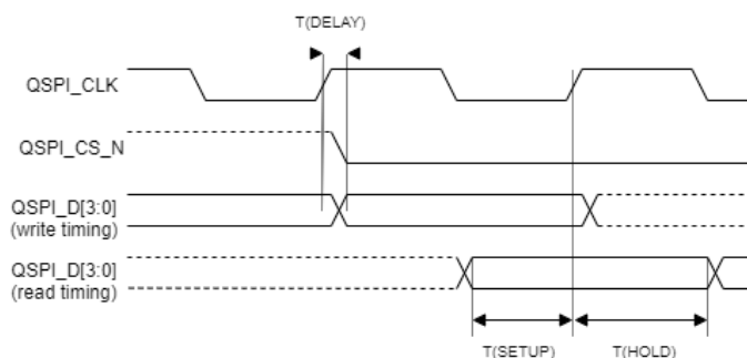
Fig. 7: QSPI Timing
