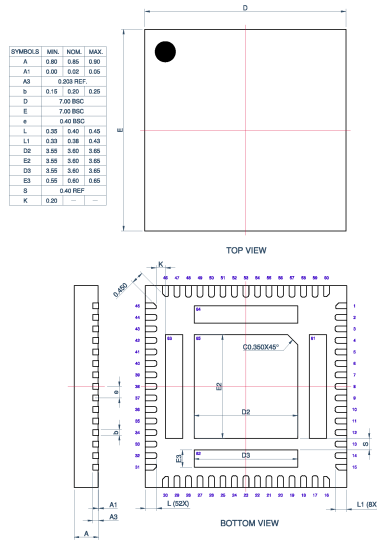
Fig. 9: Package Dimensions
