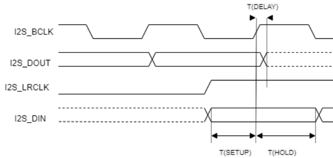
Fig. 8: I 2 S slave timing
