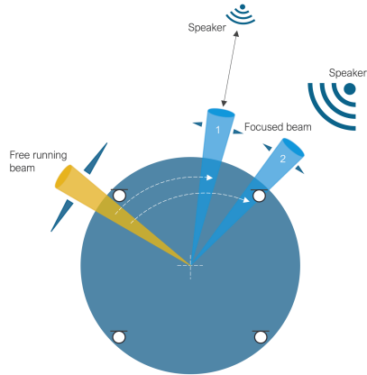
Fig. 5: Beamformer Operation
