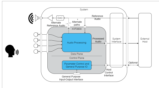
Fig. 1: XVF3800 device system context
