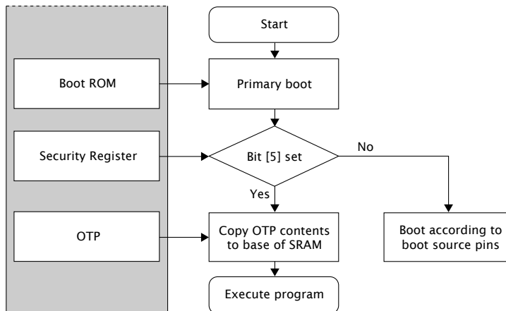
Figure 6: Boot procedure
