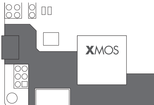
Figure 3: Integrated debugger
