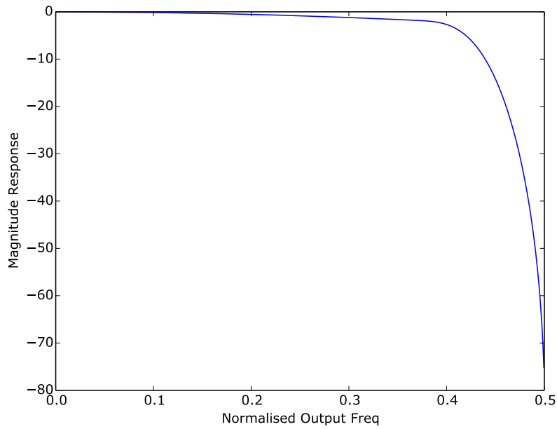
Figure 18: Final frequency response for a divide of 2.
