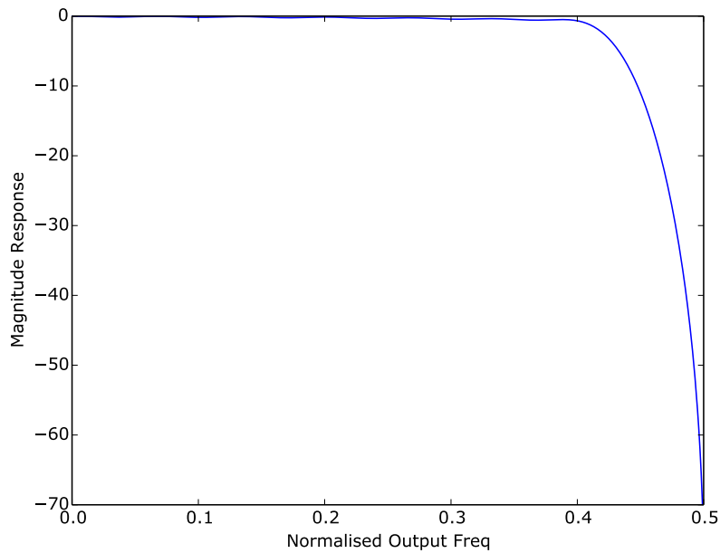
Figure 19: Final frequency response for a divide of 4.
