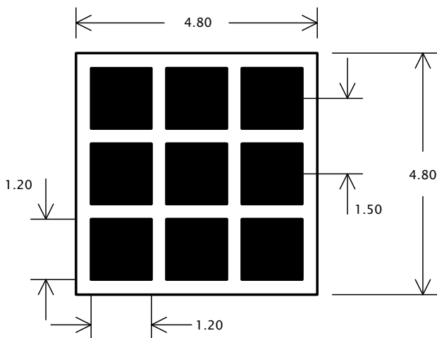
Figure 16: Solder stencil for centre pad
