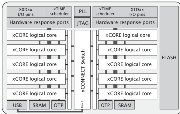
Figure 1: XUF210-256- FB236 block diagram
