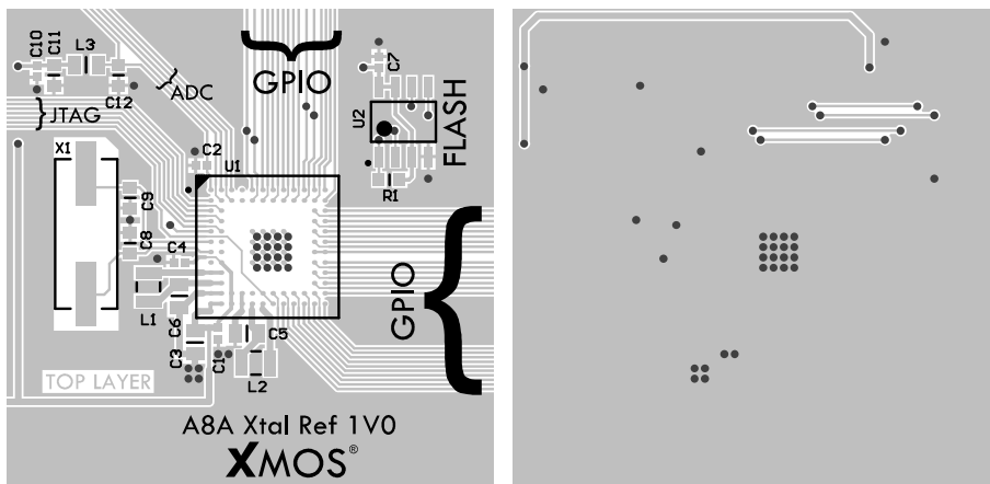
Figure 18: Example XTAL schematic, with top and bottom layout of a 2-layer PCB
