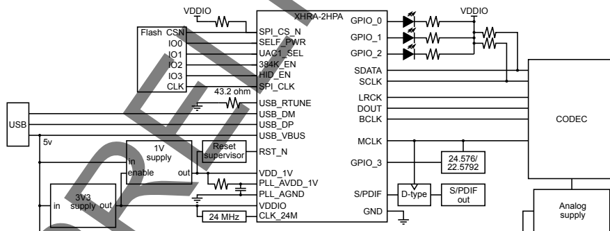
Figure 3: Simplified Reference Schematic
