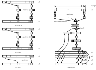
Fig. 8: Bitwise Vector load, multiply, and accumulate
