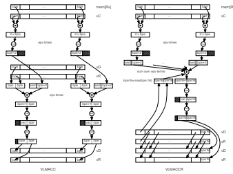
Fig. 6: Vector load and multiply accumulate operations
