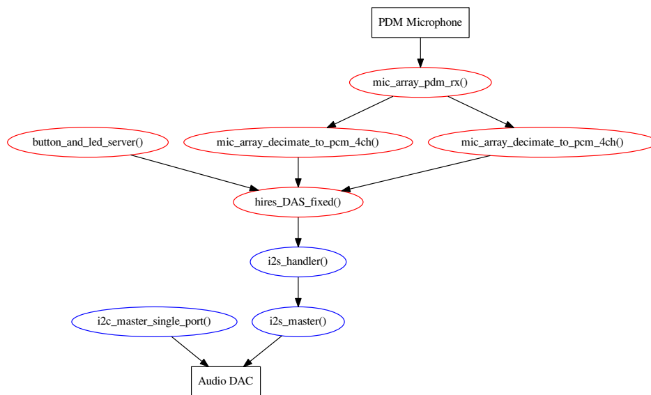
Figure 1: Application block diagram
