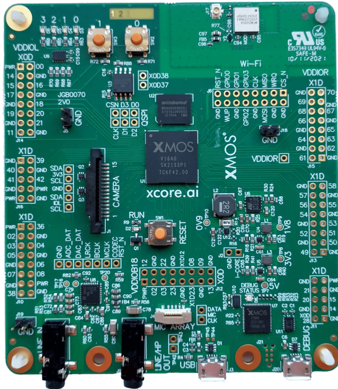
Fig. 4: XMOSES XK-EVK-XU316 Board
